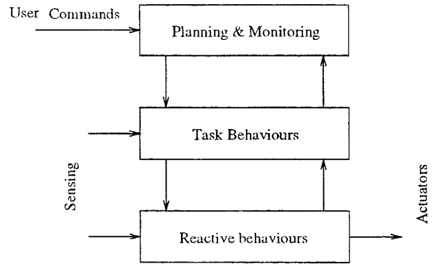
Figure 1: Overall three layer robot architecture
